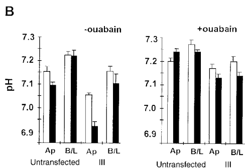
Figure 7. Several chimeras appear to be enzymatically active. The ability of chimeras to substitute for the sodium transporting activity of the endogenous Na,K-ATPase was assessed by determining whether expression of the chimera conferred ouabain resistance. All of the basolateral chimeras appears to be active as sodium pumps. However, the presence of Na,K-ATPase activity does not correlate with the steady-state distribution of the chimeras, since the apical chimera VIII confers ouabain resistance (A). The apically located chimera III also appears to be active, although it
